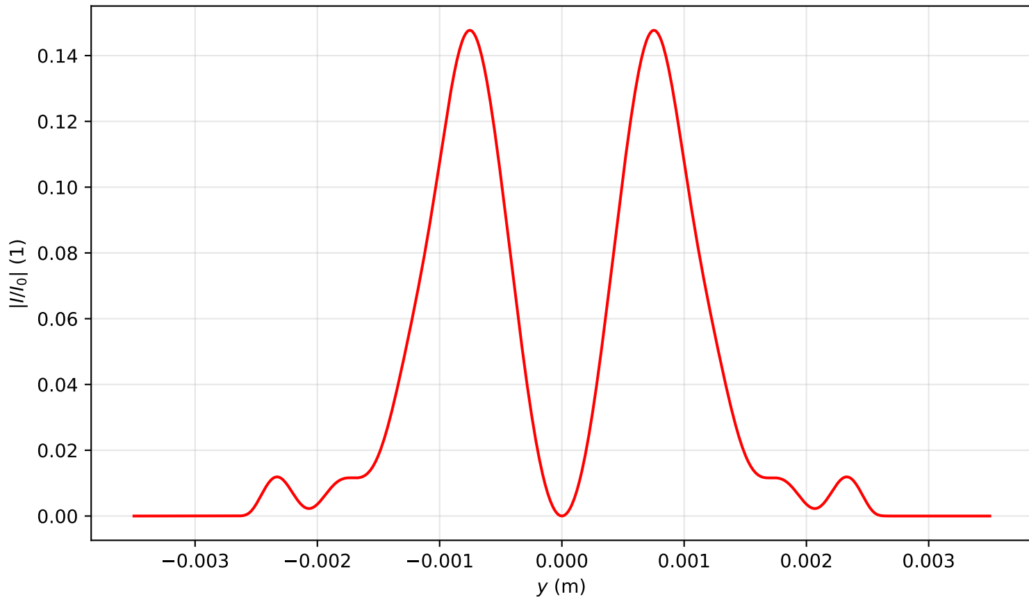
Intensity profile I(x=0, y, z=3.184)/I_0 , \text{Pin}=4.0\text{Pcr} , artificial time
